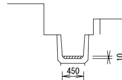
断面D L=43.0m
