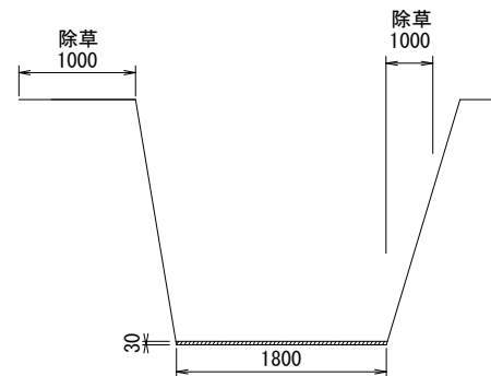
断面L L=54.0m
